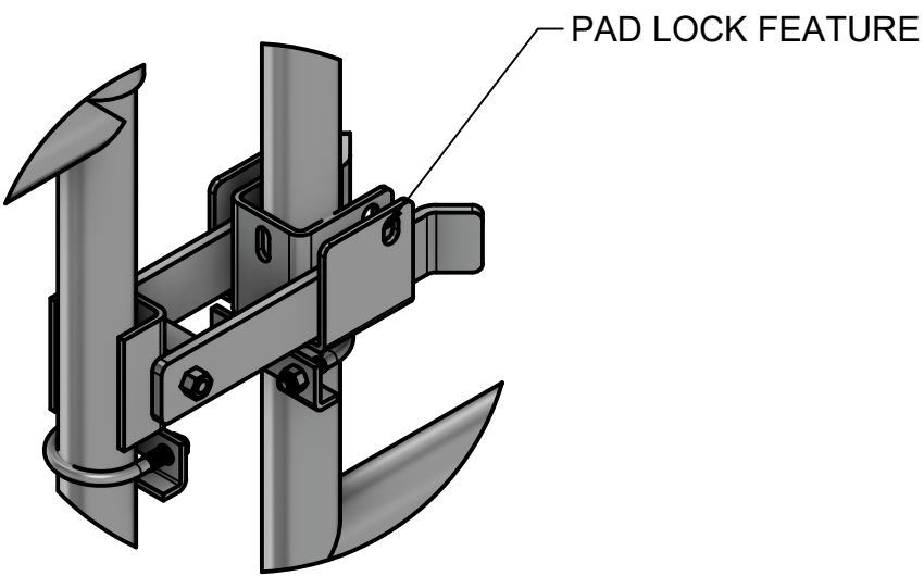
LATCH DETAIL B
